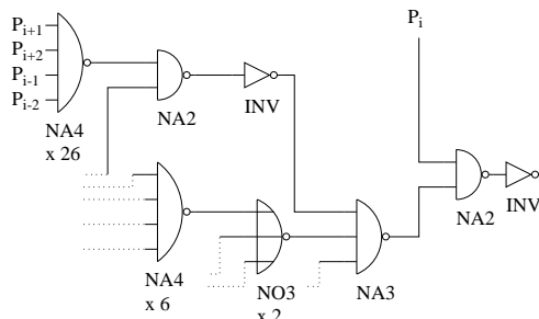
Figure 2: Schematic of a VLSI implementation for k = 2
